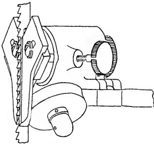
FIG. 186. BAND-SAW AND SAW GUIDES.
